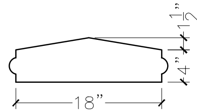
SECTION VIEW
