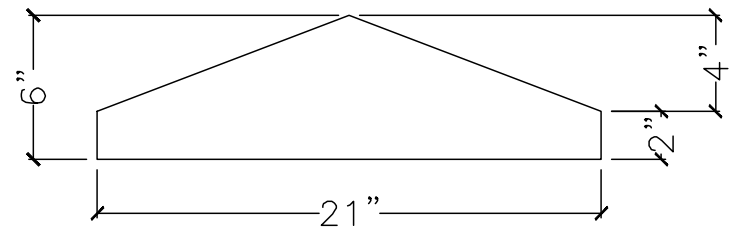
SECTION VIEW
