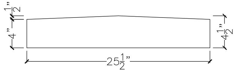
SECTION VIEW
