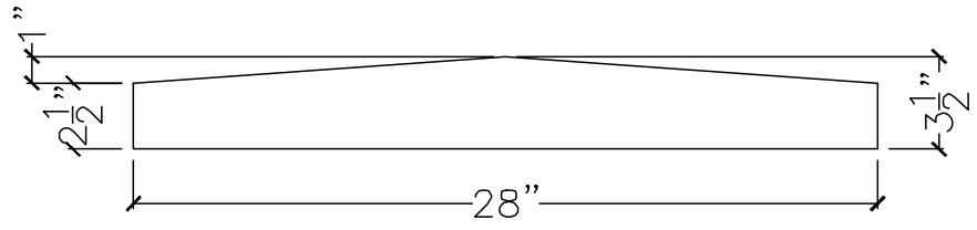
SECTION VIEW
