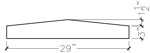
SECTION VIEW
