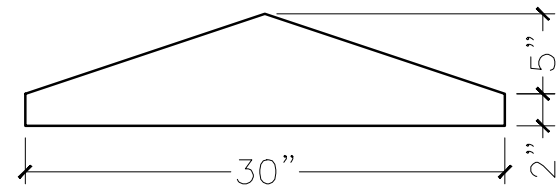
SECTION VIEW
