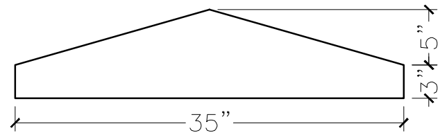
SECTION VIEW
