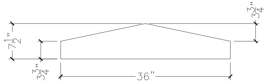
SECTION VIEW
