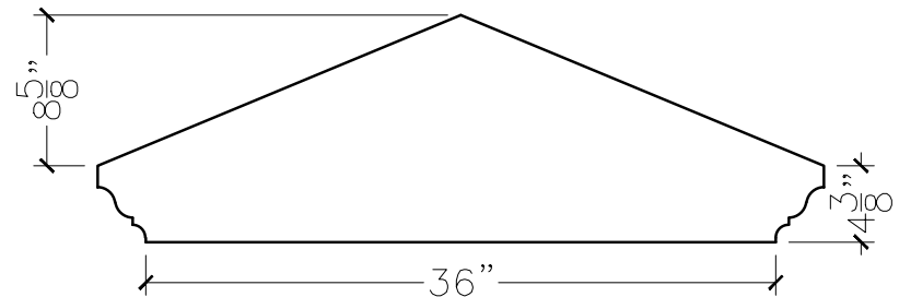
SECTION VIEW
