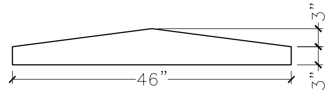
SECTION VIEW
