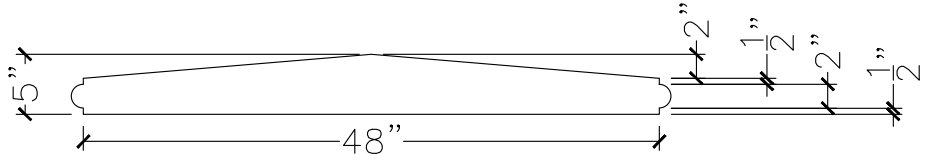
SECTION VIEW
