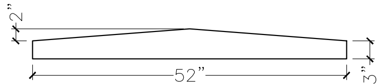
SECTION VIEW
