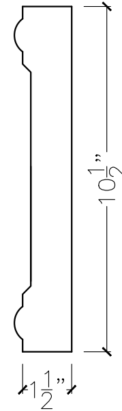
SECTION VIEW
