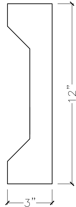
SECTION VIEW
