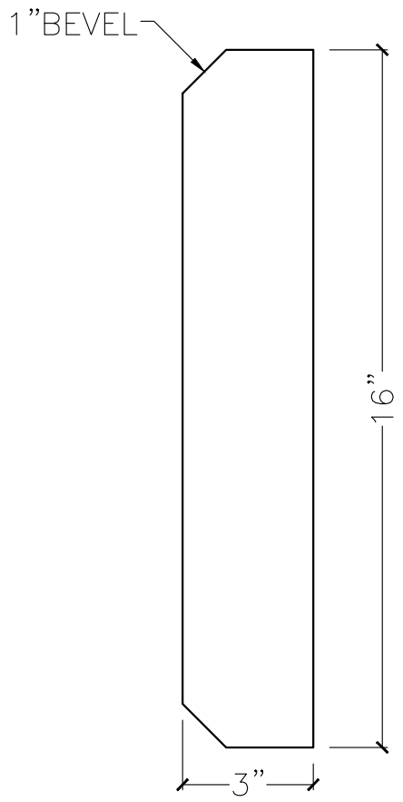
SECTION VIEW
