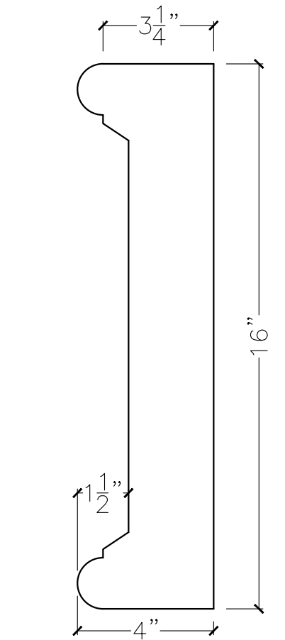
SECTION VIEW
