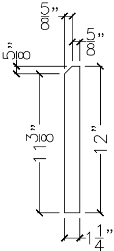
SECTION VIEW
