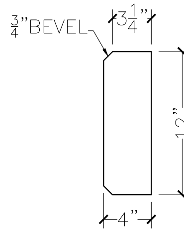
SECTION VIEW
