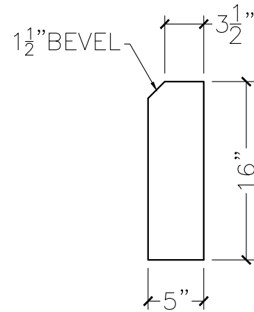
SECTION VIEW
