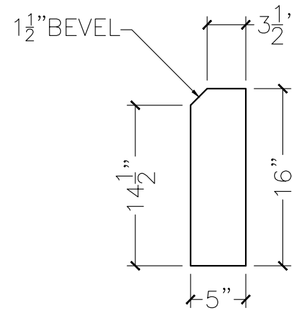
SECTION VIEW
