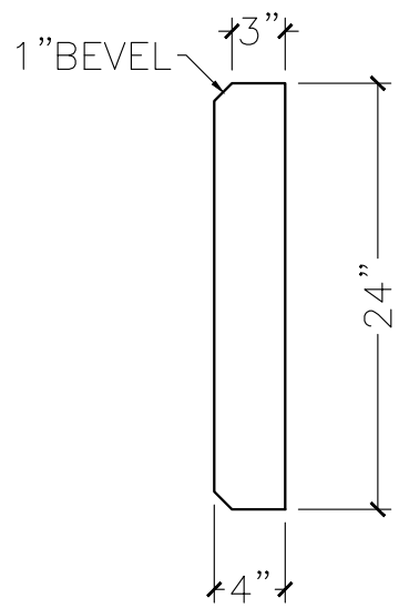
SECTION VIEW
