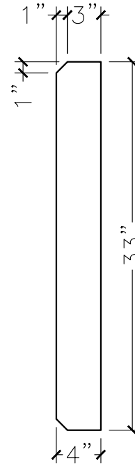
SECTION VIEW
