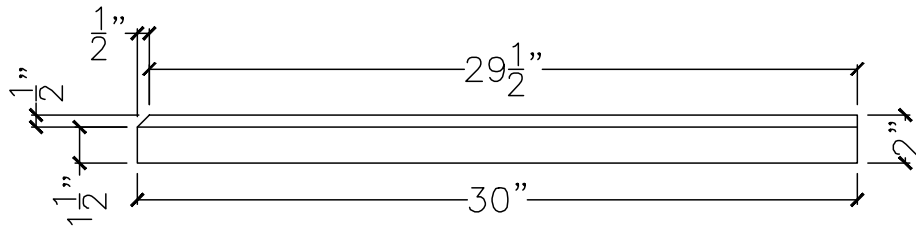
FRONT VIEW
