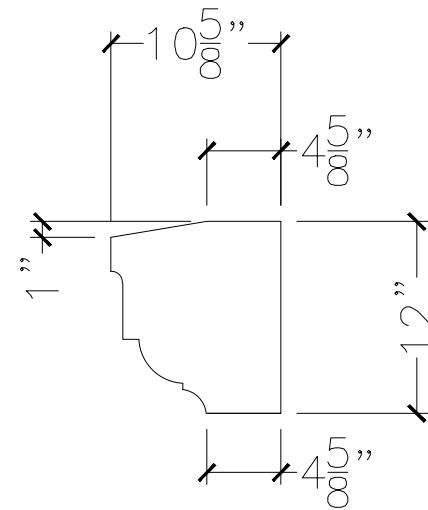
SECTION VIEW
