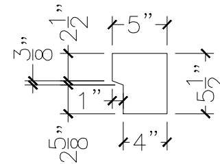
SECTION VIEW
