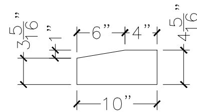
SECTION VIEW
