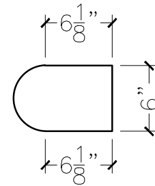
SECTION VIEW
