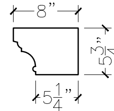
SECTION VIEW
