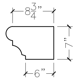
SECTION VIEW
