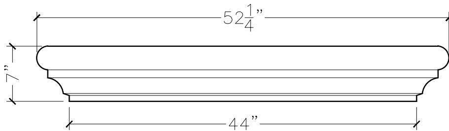
FRONT VIEW
