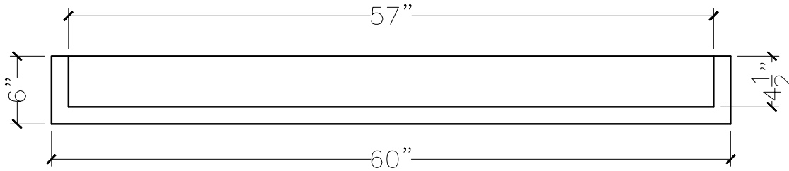
TOP VIEW
