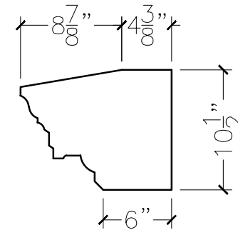
SECTION VIEW
