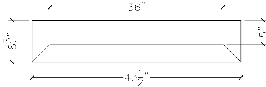
TOP VIEW
