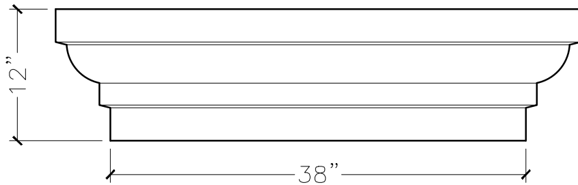
FRONT VIEW
