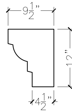
SECTION VIEW
