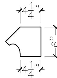
SECTION VIEW
