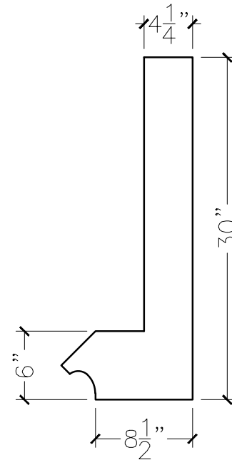
SECTION VIEW
