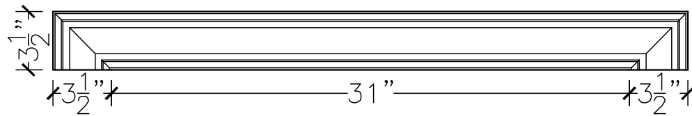
FRONT VIEW
