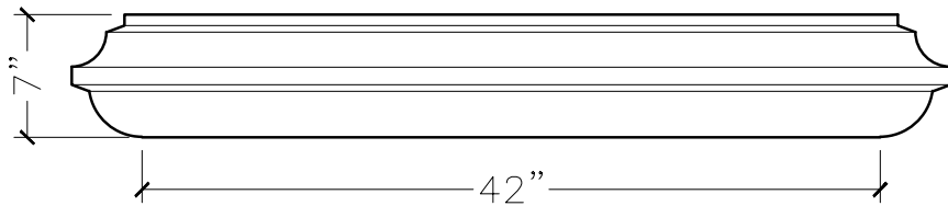
FRONT VIEW
