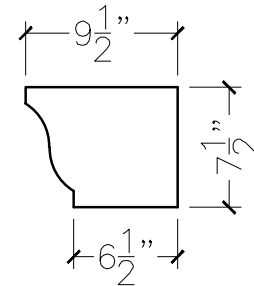
SECTION VIEW
