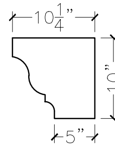
SECTION VIEW
