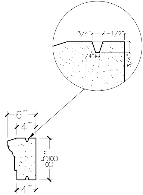
SECTION VIEW
