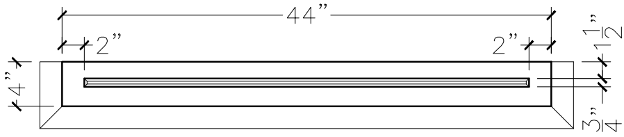
TOP VIEW
