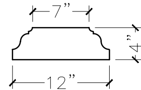
SECTION VIEW
