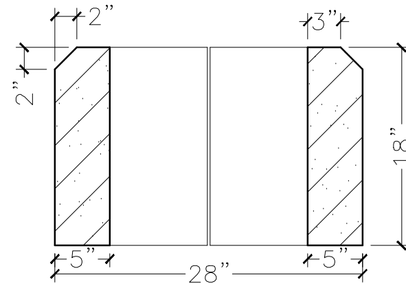
SECTION VIEW
