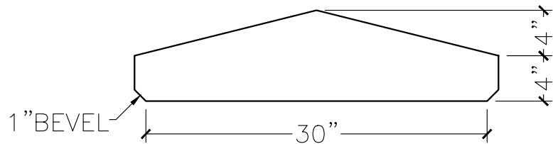
SECTION VIEW
