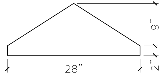
SECTION VIEW
