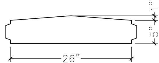
SECTION VIEW
