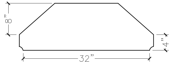
SECTION VIEW
