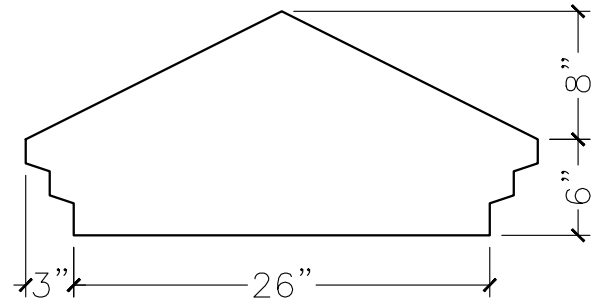
SECTION VIEW
