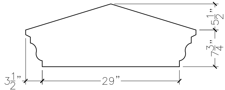
SECTION VIEW
