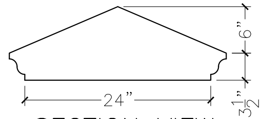
SECTION VIEW
